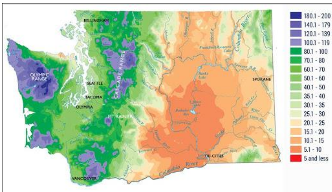
FIGURE 12: ANNUAL PRECIPITATION IN WASHINGTON STATE 28
