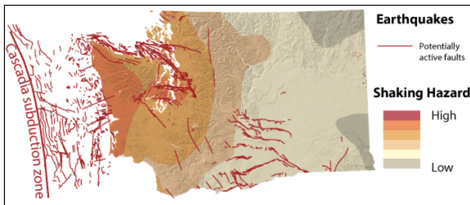
FIGURE 9: SEISMIC RISK FROM HIGH TO LOW AND POTENTIALLY ACTIVE FAULTS IN WASHINGTON 20
